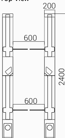
Top View
