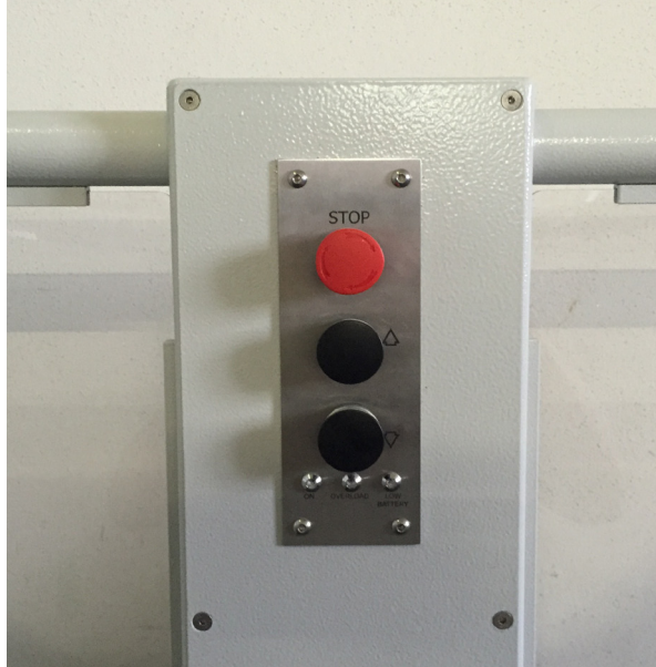
Controls on the platform with stop button, as well as LED indication of overload and low battery voltage
