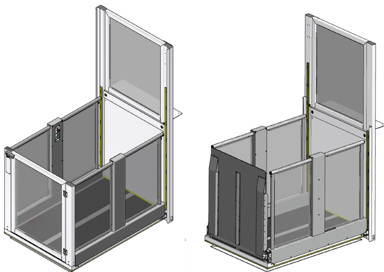
Schematic views of units with a door on the platform and with a access ramp on the platform
